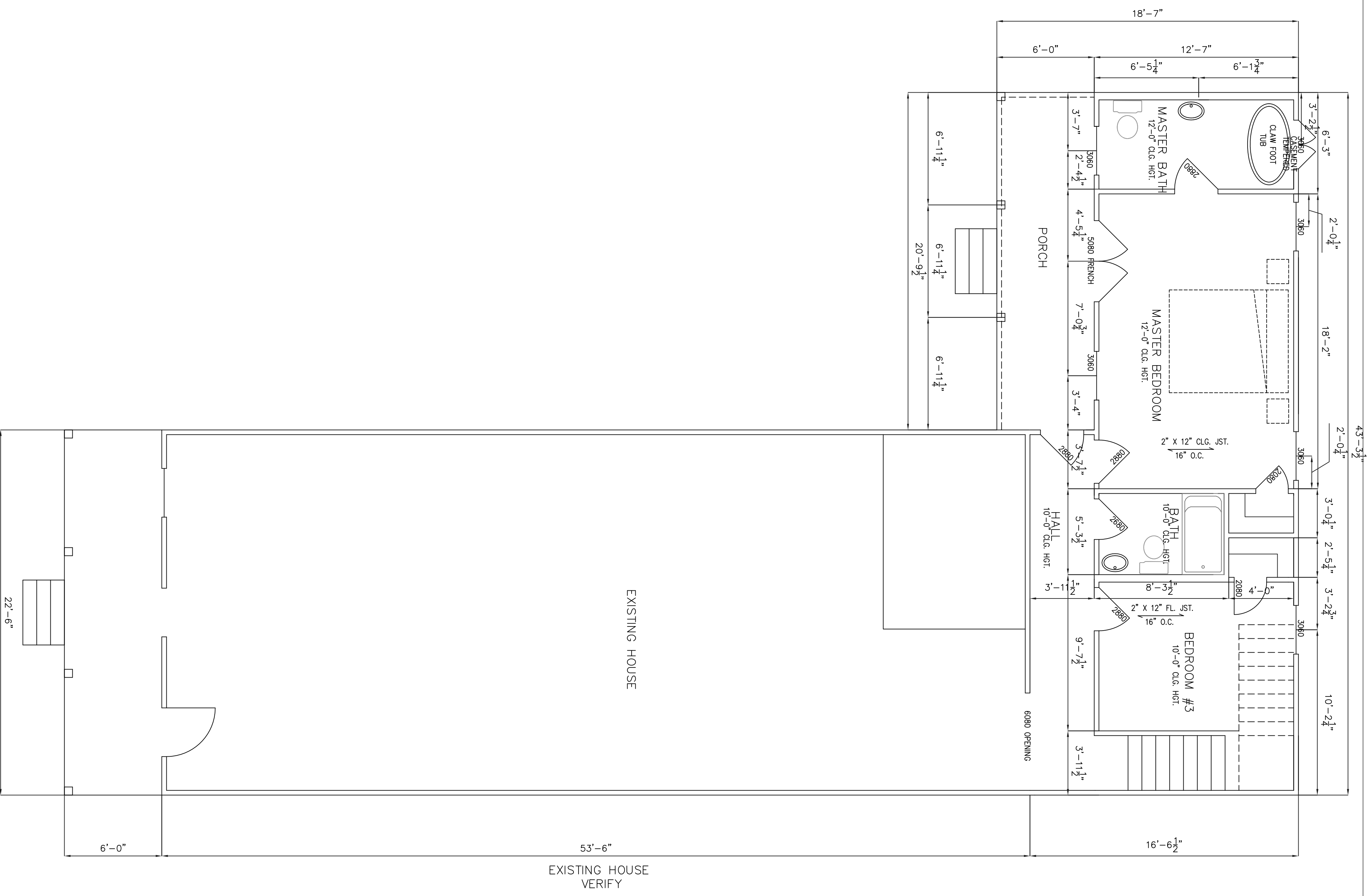
1. FLOOR PLAN 1/4" = 1'-0"
